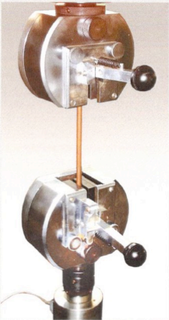
Wedge Grips for Flat & Round Specimens
