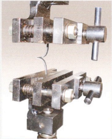
Screw Grip for Peel Test
