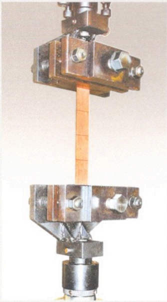
Screw Grip for flat Specimens
