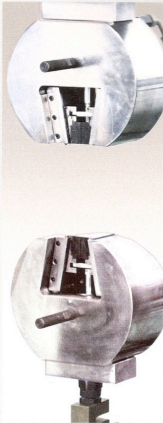
Hydraulic Wedge action grips for round & flat specimens
