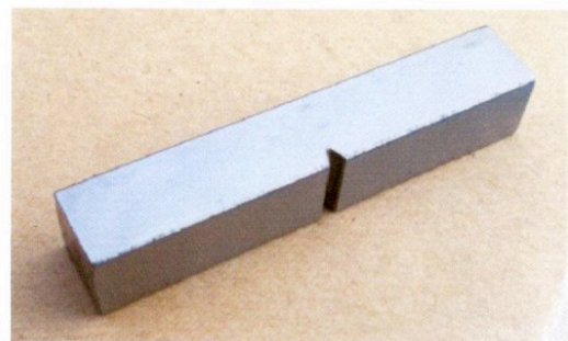
Standard Specimen
